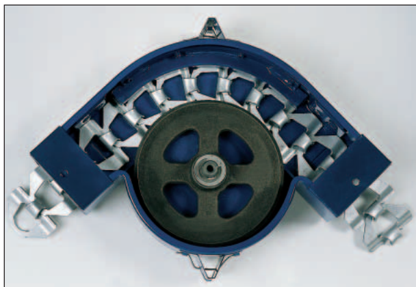
90° corner with CHAMPION feed chain
